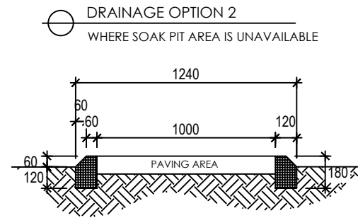
○ CURB STONE AND PAVING AREA SECTION DETAIL
