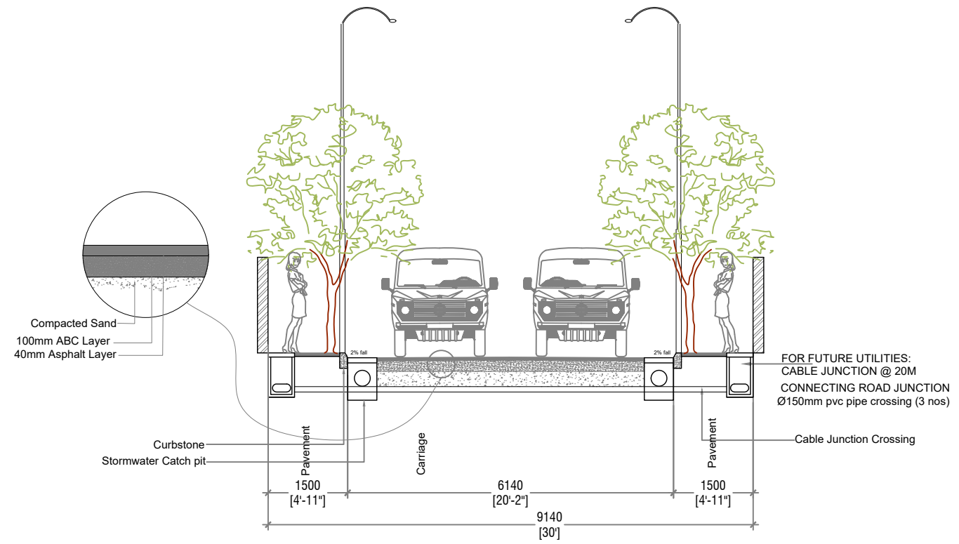
KAAMINEE MAGU - SECTION (9.14M)
