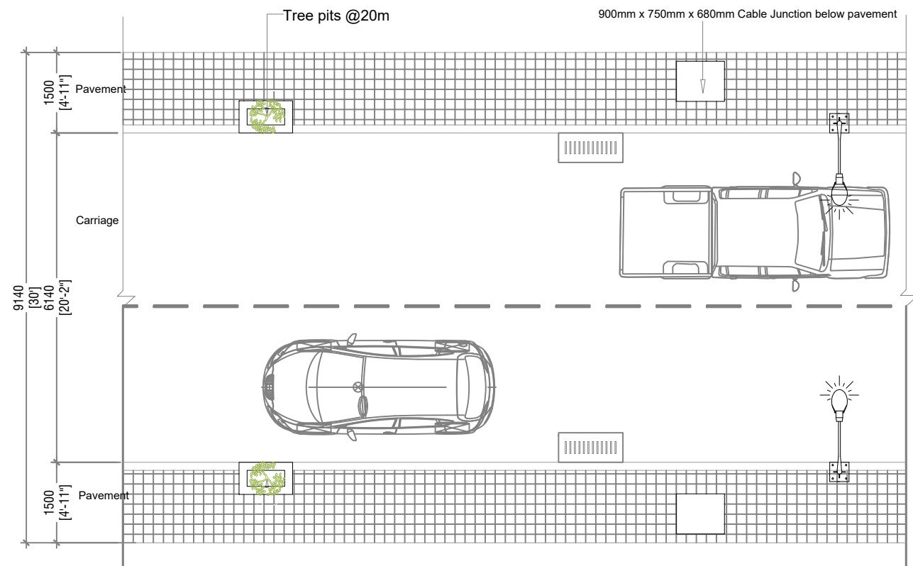
9.14M ROADS - PLAN
