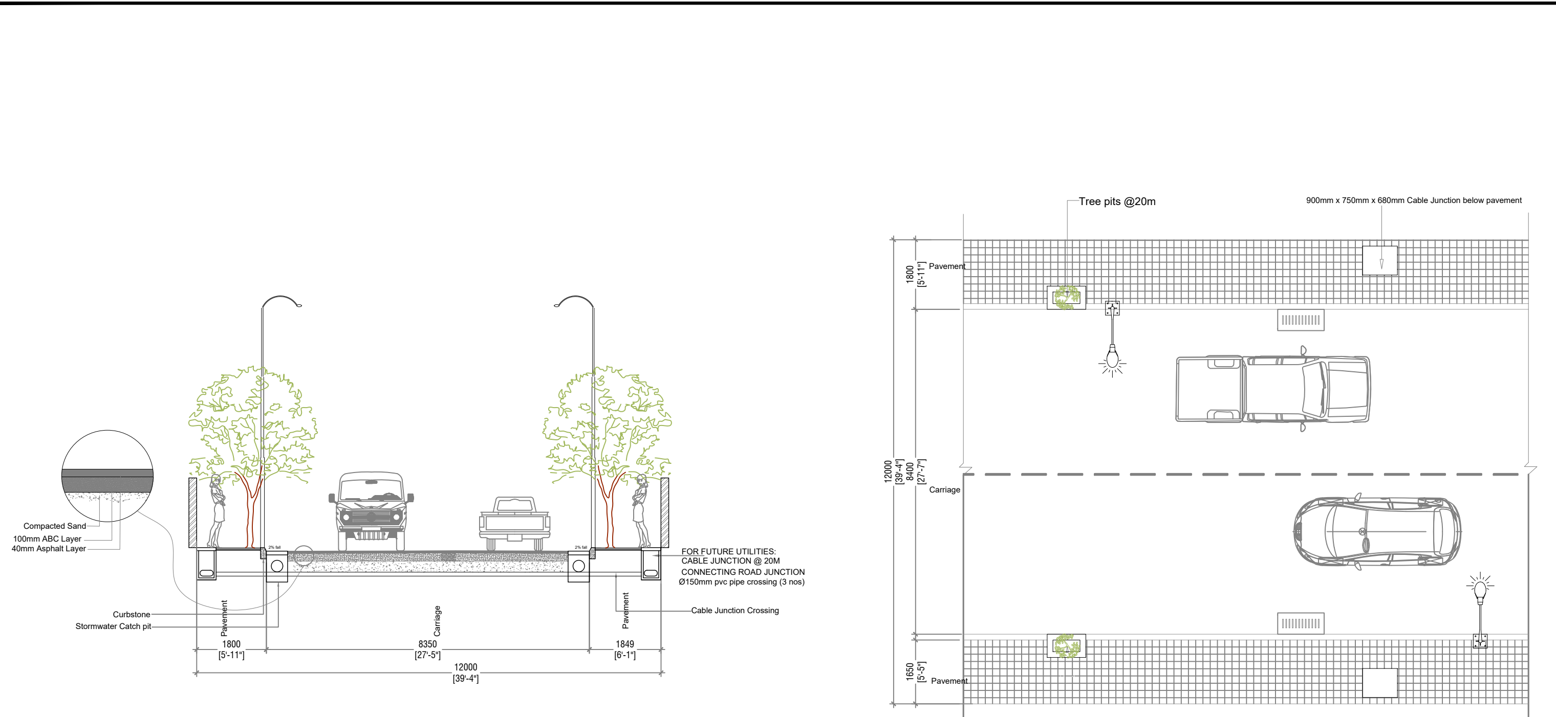
NOORAANEE MAGU - SECTION (12M)
