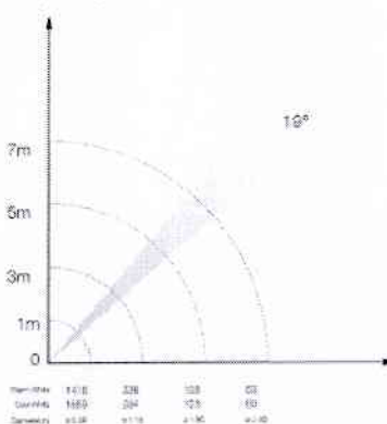
Light Output (FC=LUK × 0.0029)
