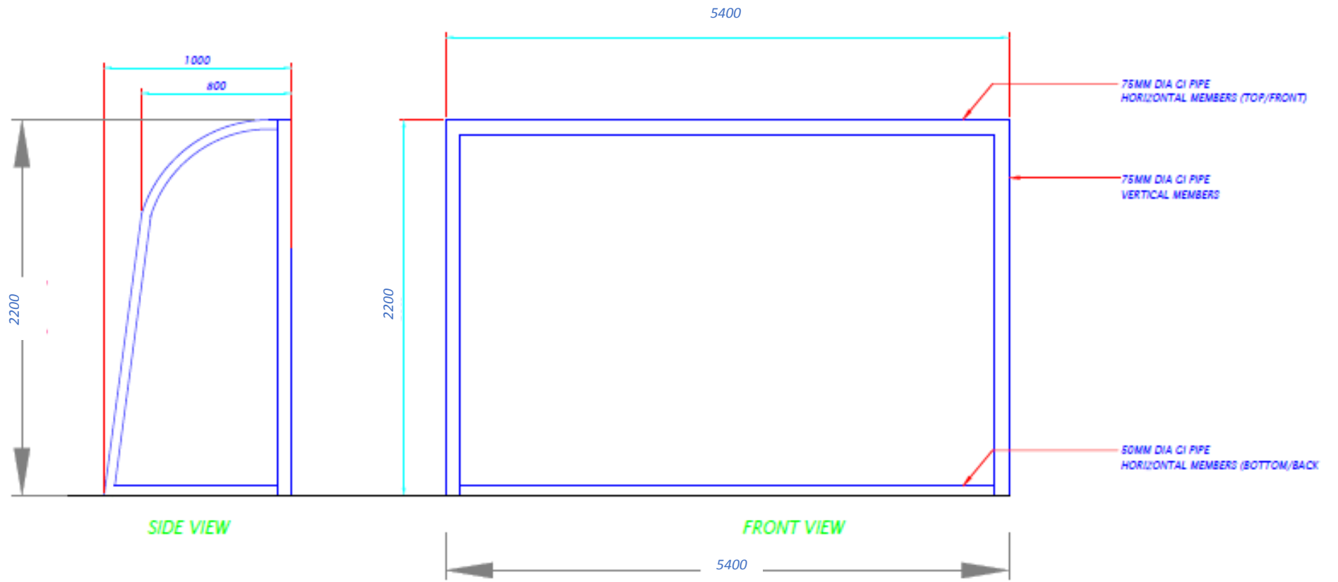
DETAL-GOAL POST Scale - 1:20
