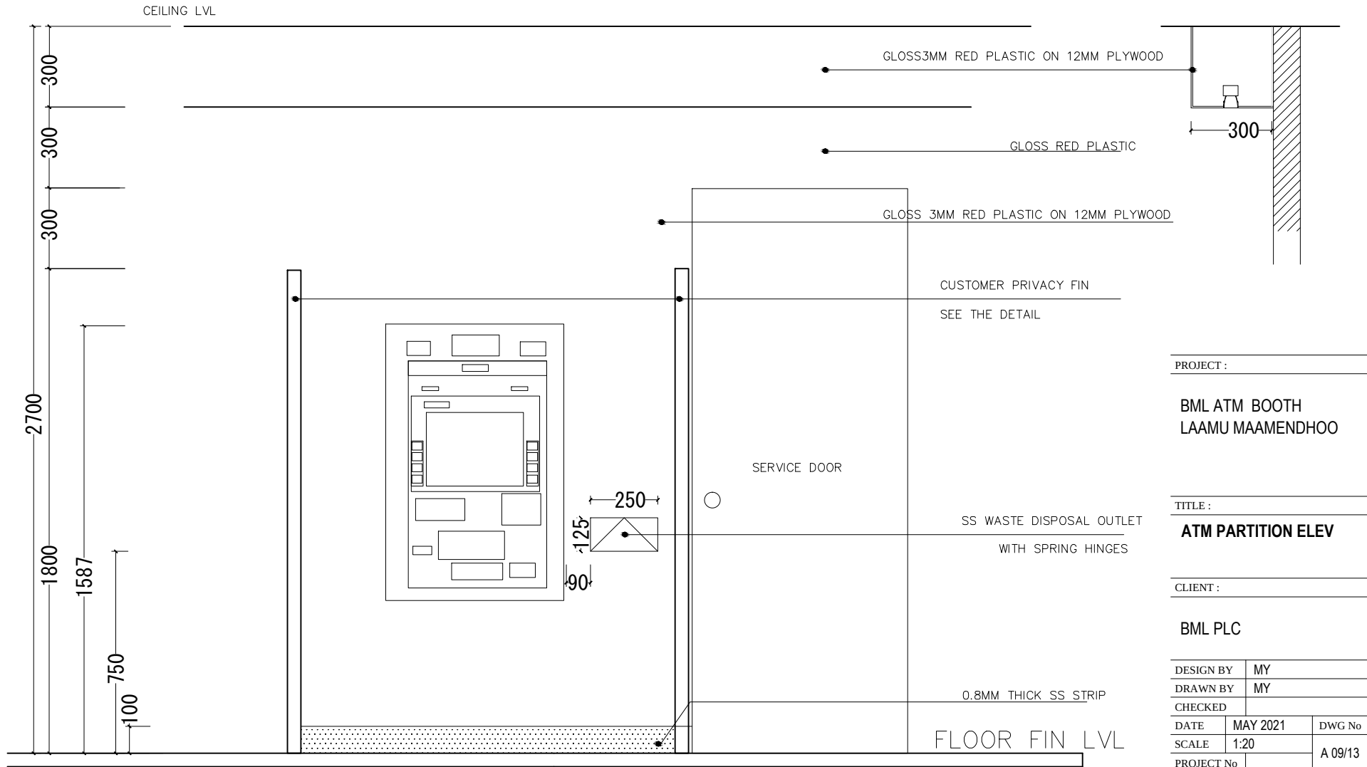
EVEVATION - E1 SCALE 1:20
