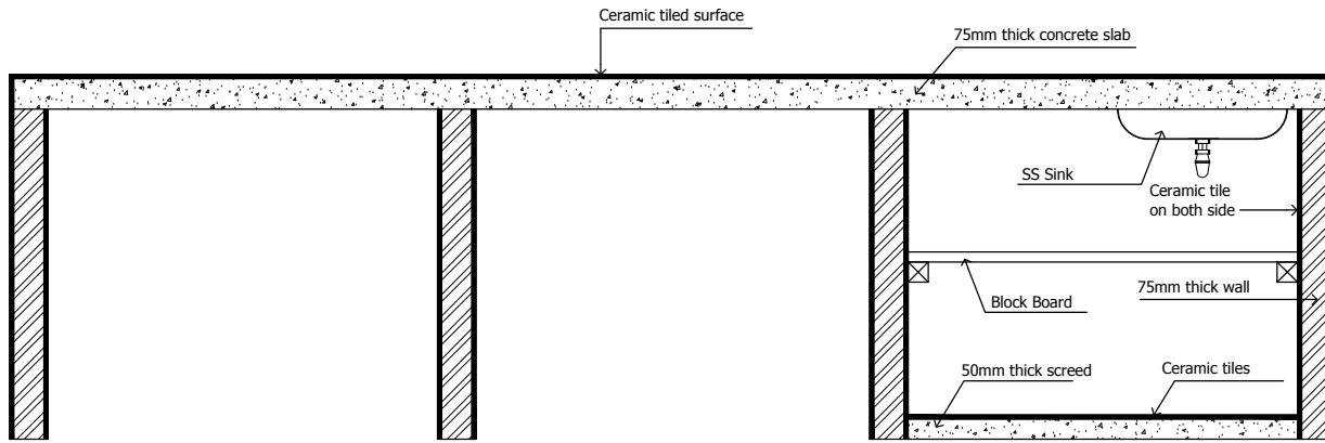
SINK STRUCTURE DETAIL
