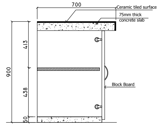
SINK CUPBOARD SECTION B - B
