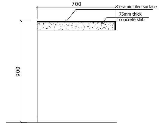
SINK CUPBOARD SECTION A-A
