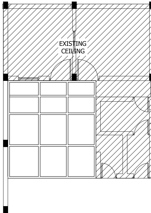
CEILING LAYOUT
