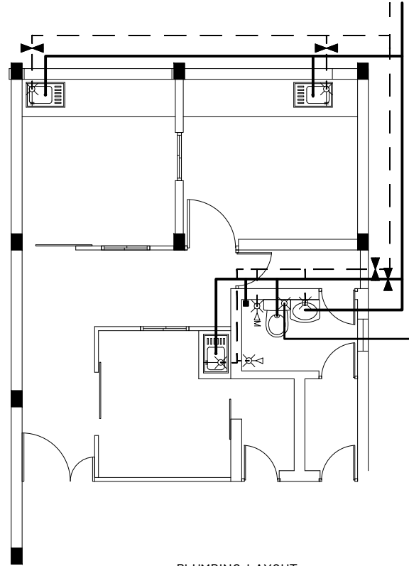
PLUMBING LAYOUT
