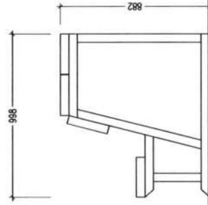
PORTABLE PLAYERS BENCH- SIDE ELEVATION SCALE 1:20
