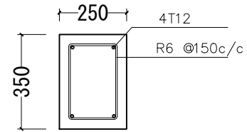
FOUNDATION BEAM
