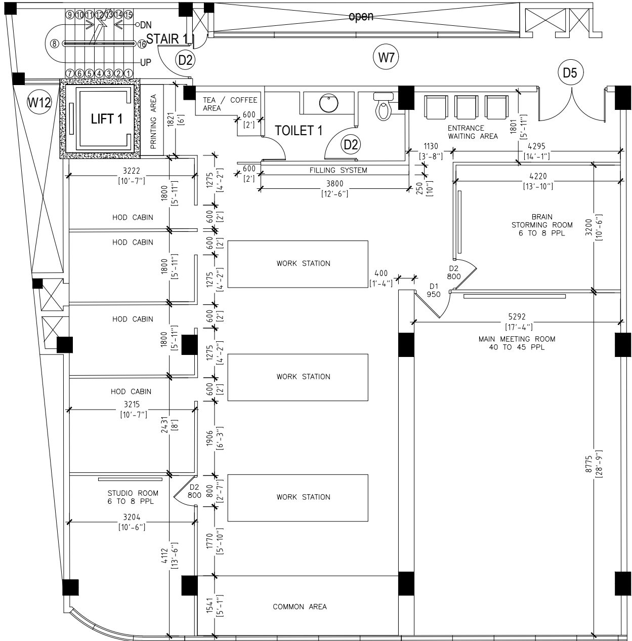
FLOOR DIMENSIONS MMPRC OFFICE
