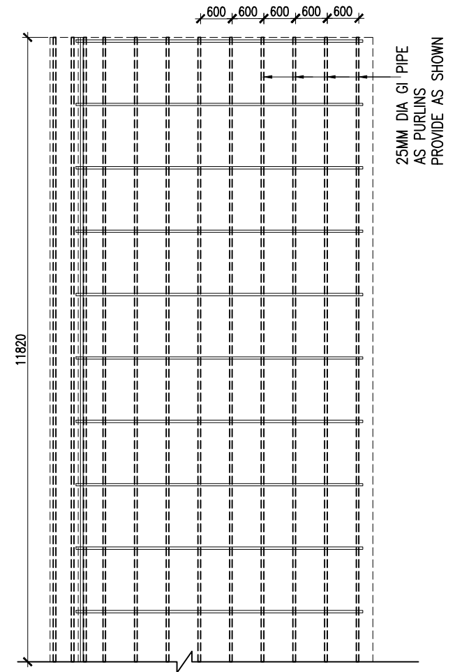
HALF PURLINS PLAN OF WASTE COLLECTION SHED
