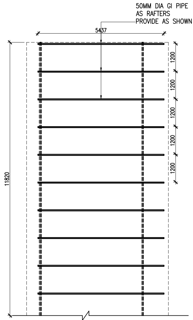
HALF RAFTER PLAN OF WASTE COLLECTION SHED
