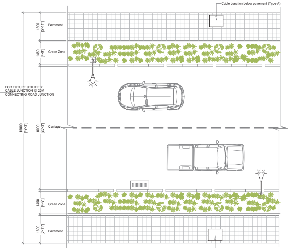
15M ROAD - PLAN
