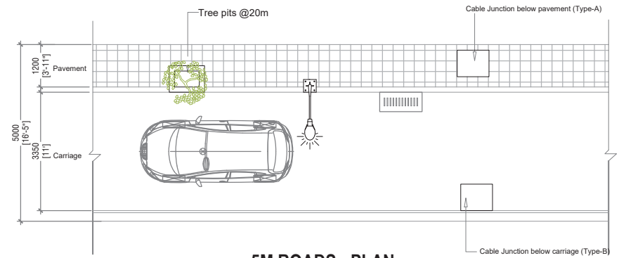
5M ROADS - PLAN
