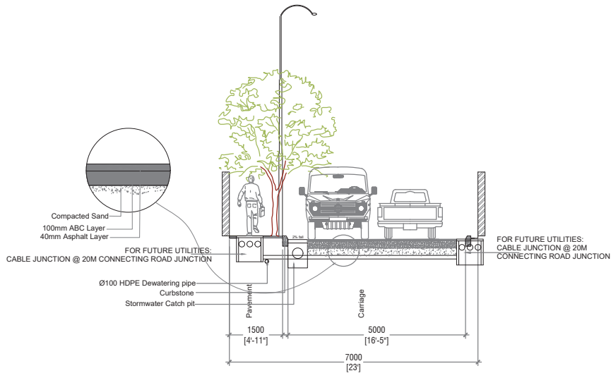
SAIMAA HIGUN - SECTION (7M)
