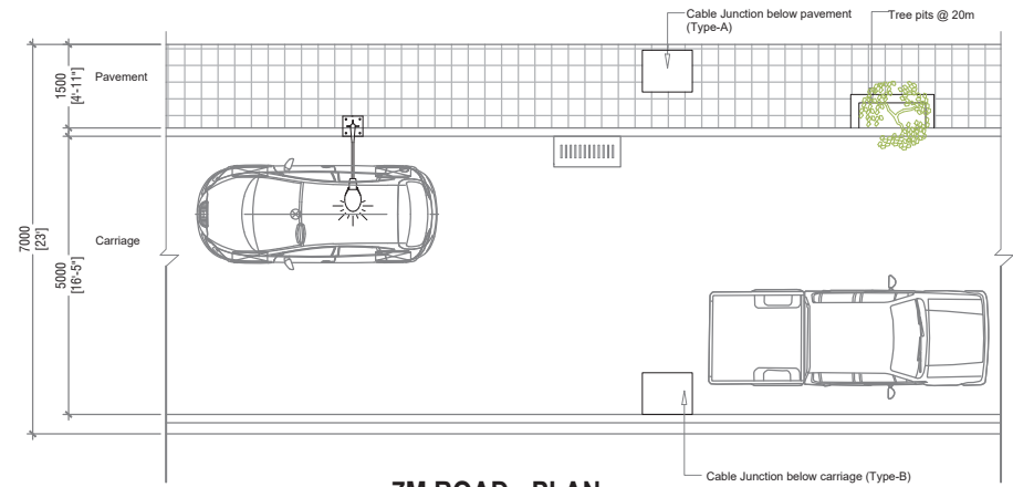
7M ROAD - PLAN
