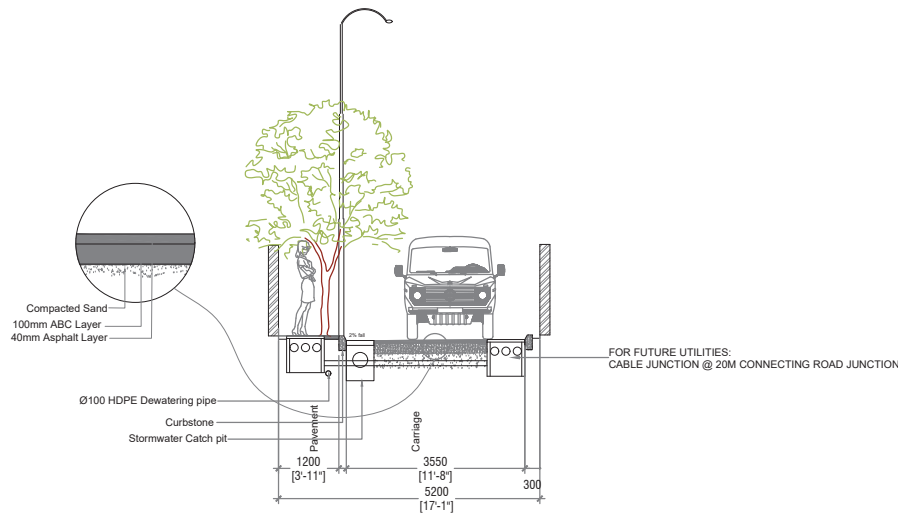
SHAHEED ALI HIN'GUN - SECTION (5.2M)
