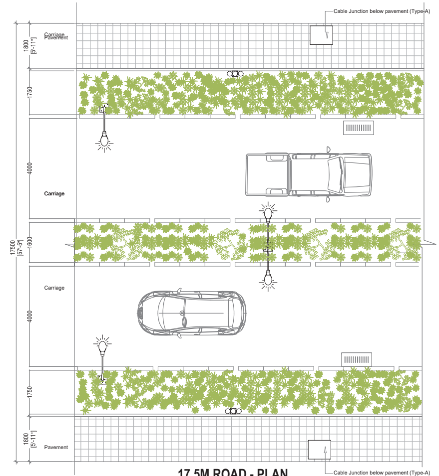
17.5M ROAD - PLAN
