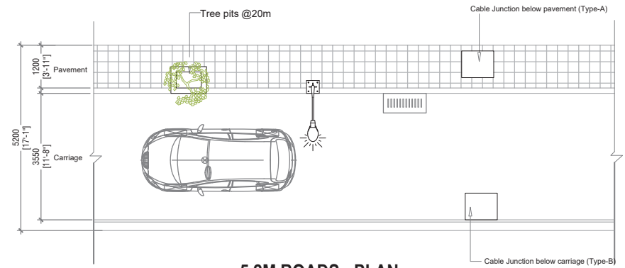
5.2M ROADS - PLAN
