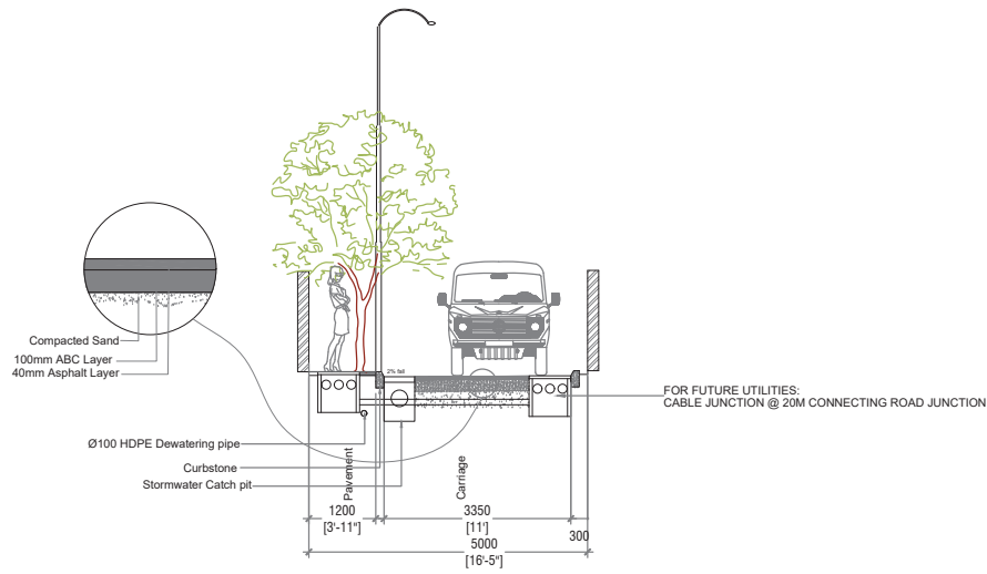
KARIYYA MAGU - SECTION (5M)
