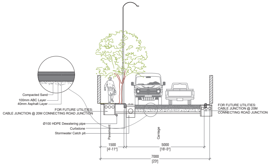
BANDHARU MAGU - SECTION (7M)
