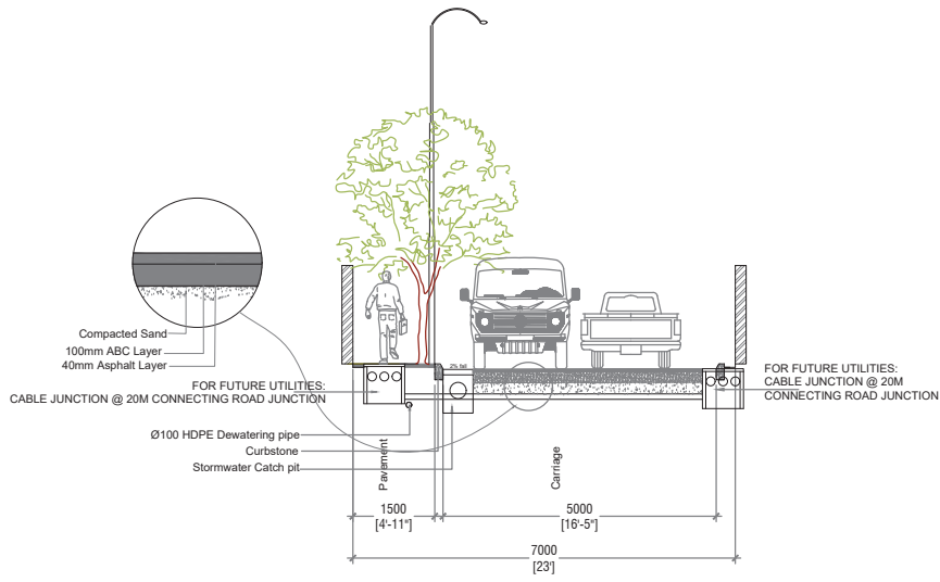
BALLEEDHANDU HIN'GUN - SECTION (7M)
