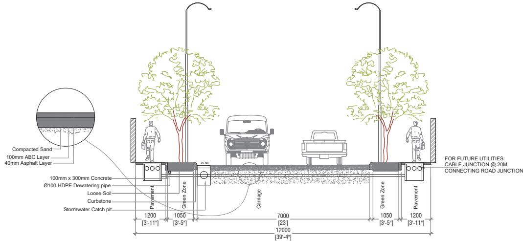
RAIVILLA MAGU - SECTION (12M)
