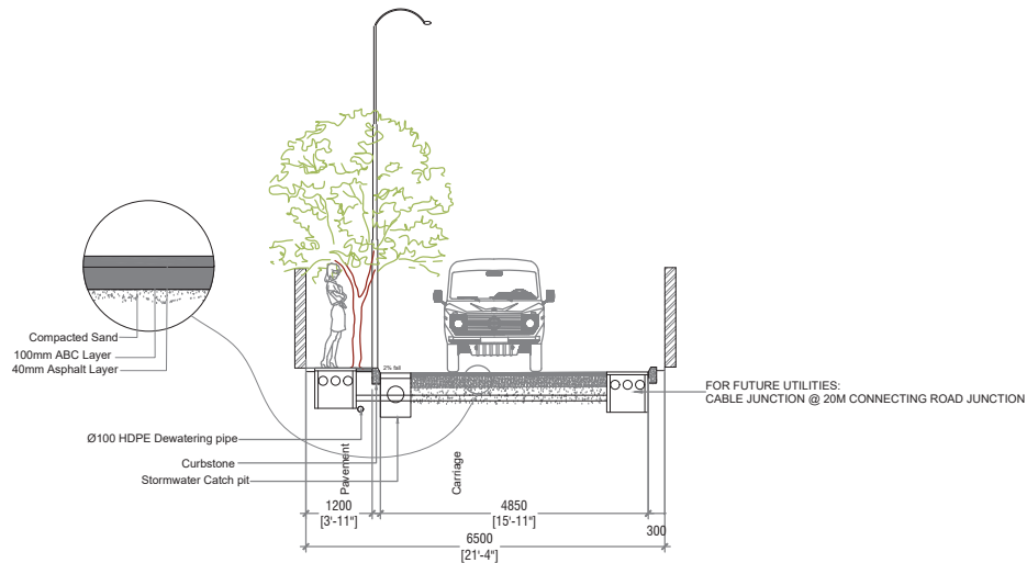
HUSEINEE HIN'GUN - SECTION (6.5M)
