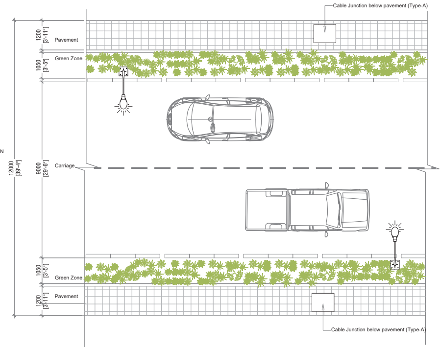
12M ROAD - PLAN
