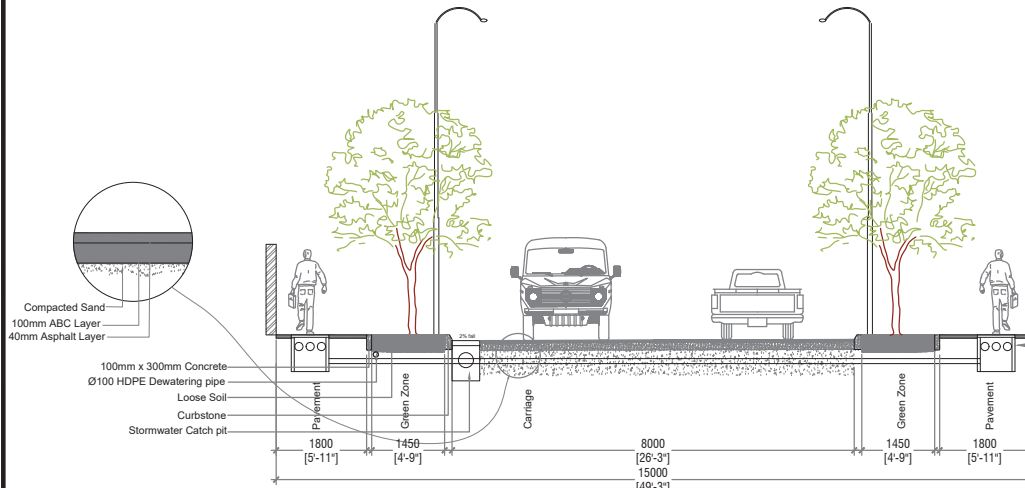
DHOSHIMEYNA MAGU - SECTION (15M)
