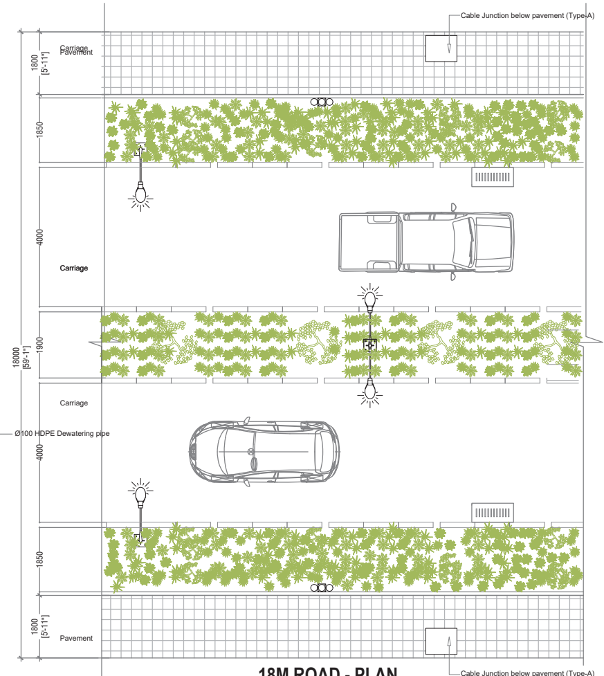
18M ROAD - PLAN
