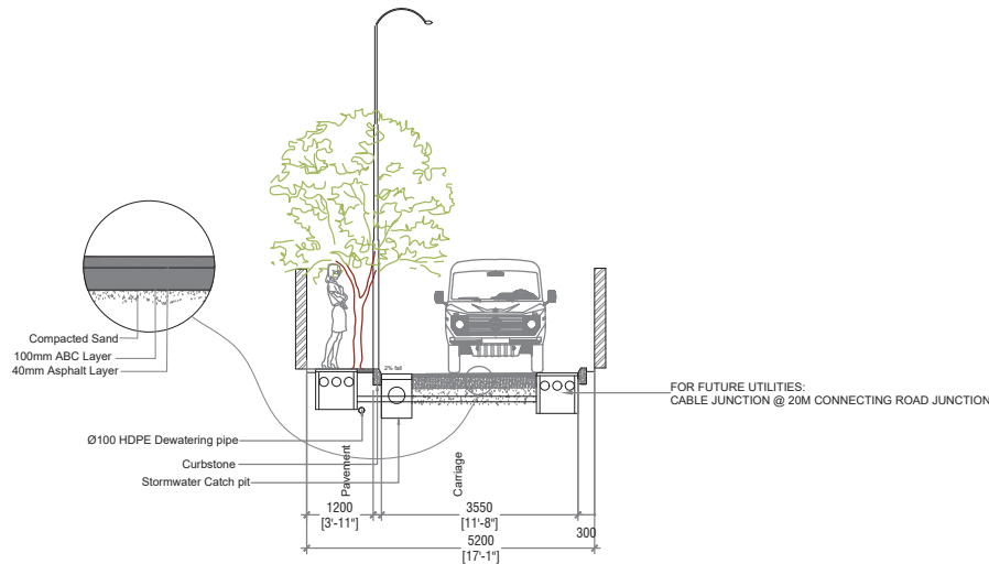
MOONIMAA MAGU - SECTION (5.2M)
