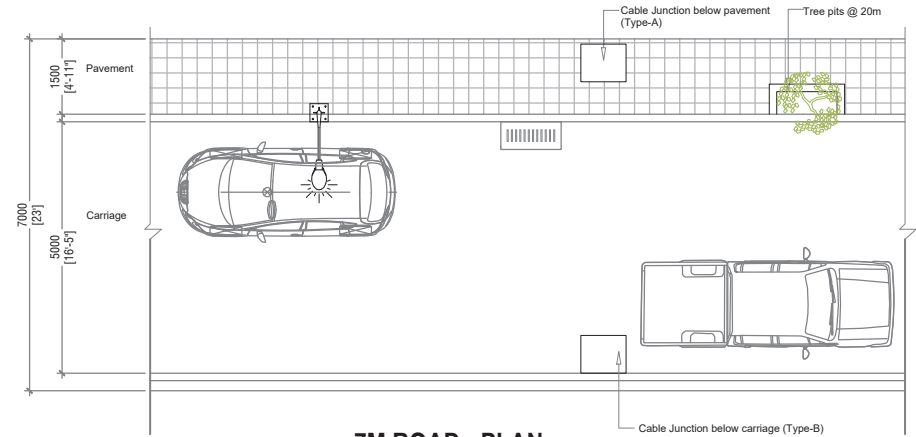
7M ROAD - PLAN SCALE 1:100
