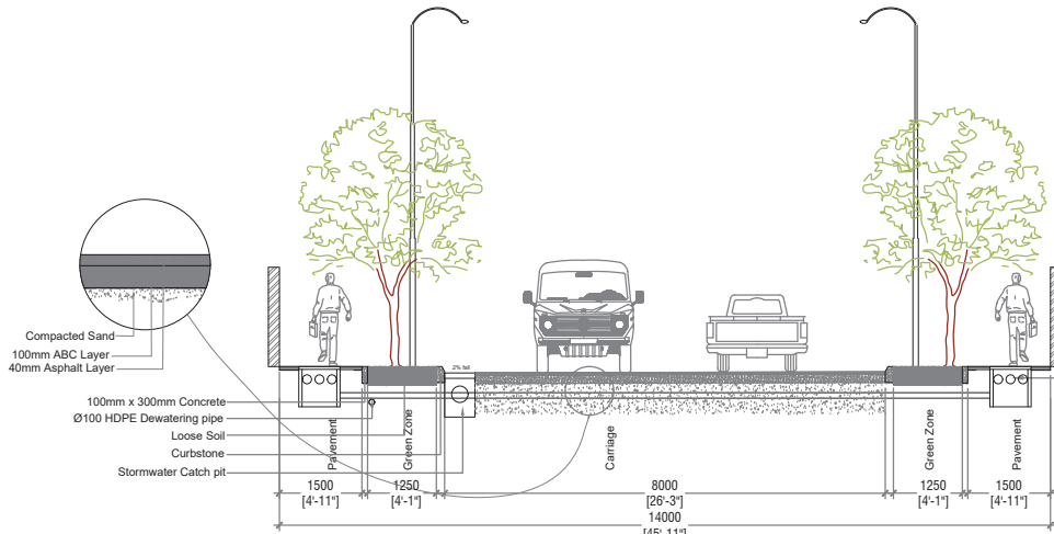
RAVILLA MAGU - SECTION (14M)
