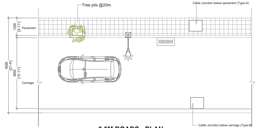
6.5M ROADS - PLAN
