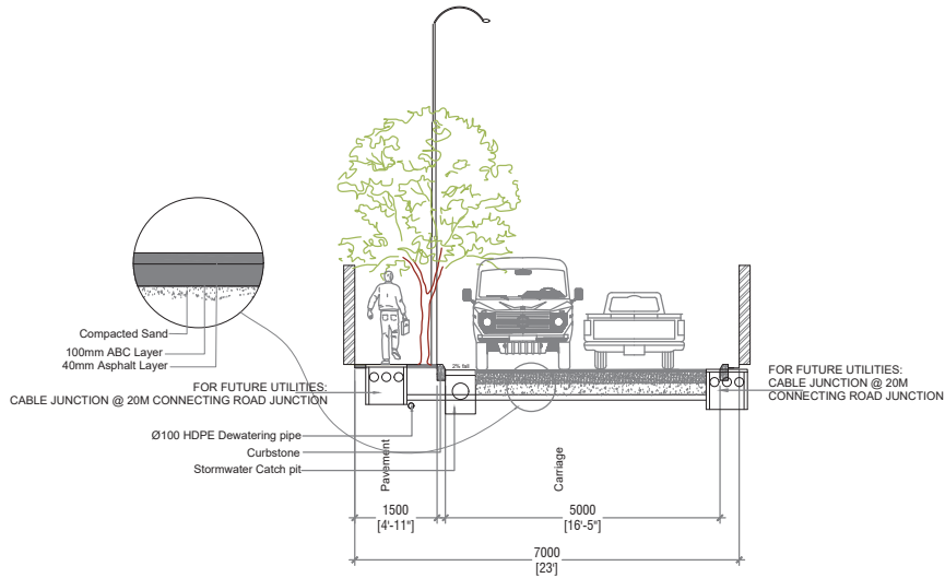
SITHIMAVAARANI HIN'GUN - SECTION (7M)
