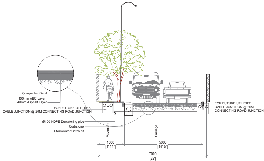
KAASHINJEE HIN'GUN - SECTION (7M) SCALE 1:100
