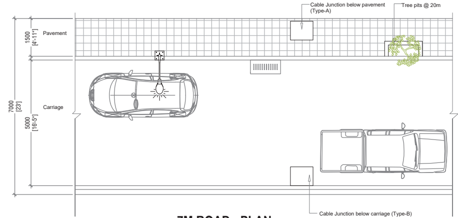
7M ROAD - PLAN
