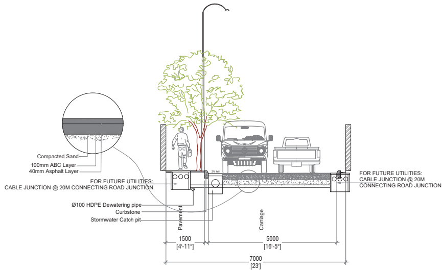
THUNDEE GOALHI - SECTION (7M)
