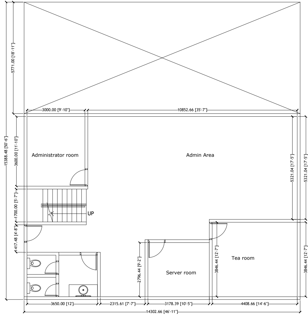
FIRST FLOOR
