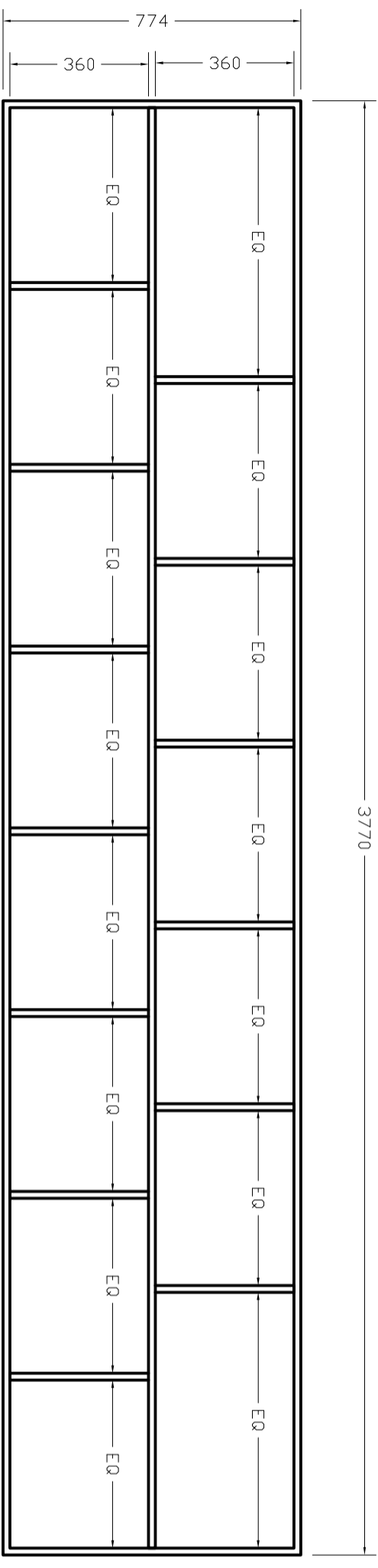
SHELF-2 FRONT ELEVATION 1:15
