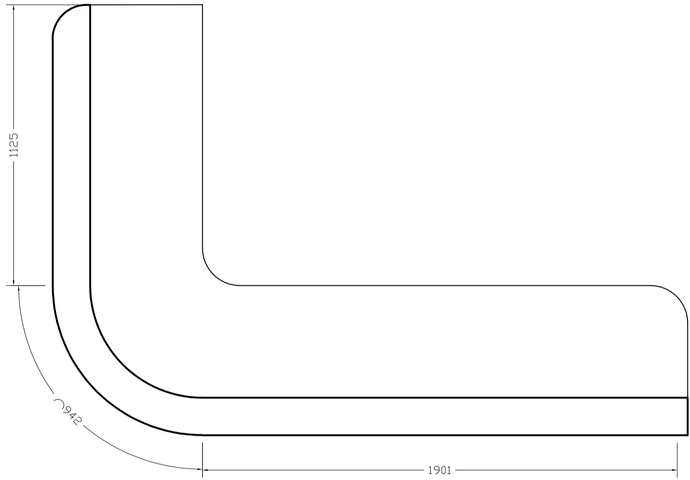
RECEPTION COUNTER PLAN 1:15
