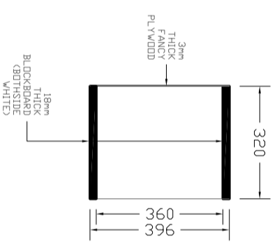
SHELF-3 SECTION Y-Y 1:10
