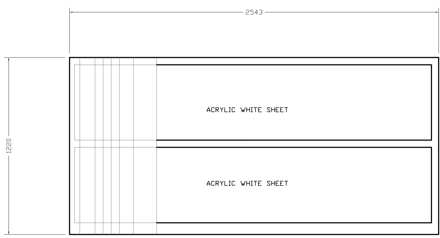
RECEPTION COUNTER PLAN 1:15
