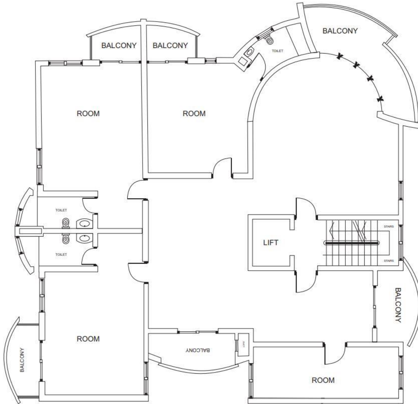
H. HULHUGALI 5TH FLOOR PLAN
