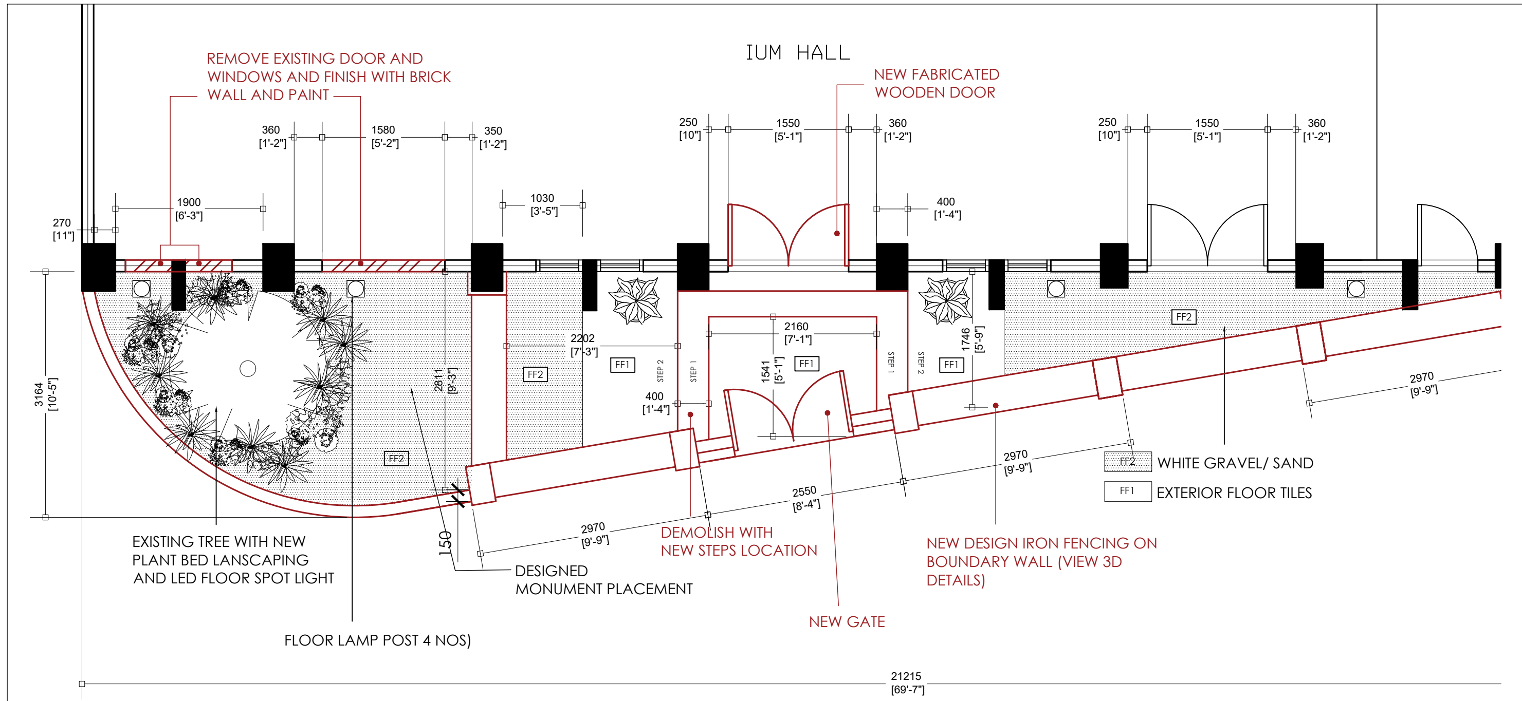
BOUNDARY NEW PROPOSED PLAN SCALE: 1:50
