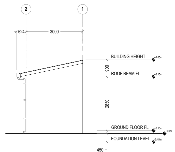
2 SIDE ELEVATION REF. HAZARDOUS BUILDING SCALE : 1:100 (A3)
