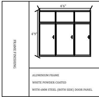
WINDOWS DETAILS
