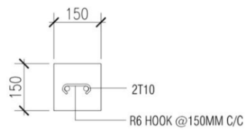
LINTEL BEAM
