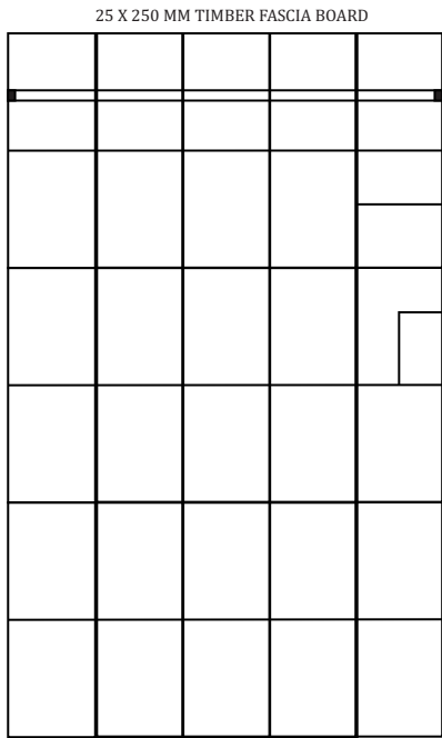
ROOF FRAMING PLAN
