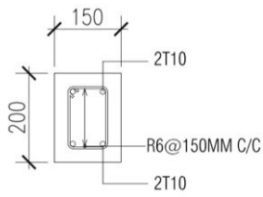
COLUMN DETAILS SCALE 1:10
