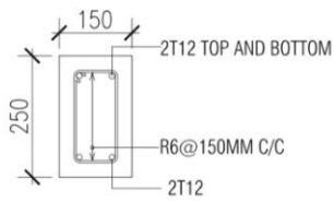
ROOF BEAM DETAILS
