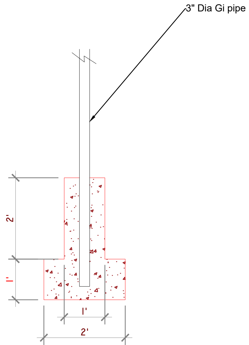
EXISTING FENCE POST
