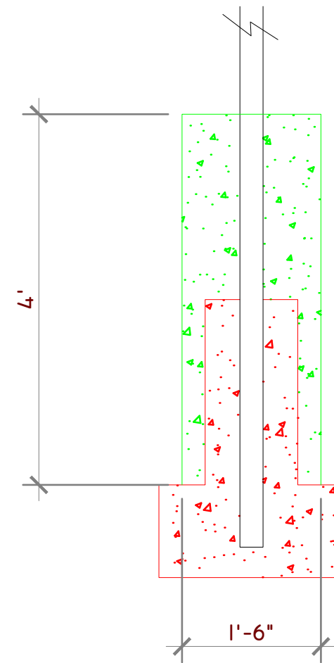
FENCE POST AFTER RE-ENFORCEMENT
