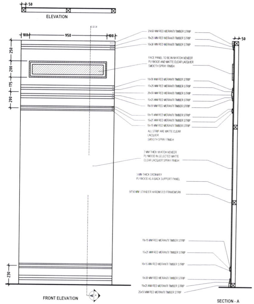
AR 2/5 SCALE COURT ROOM BACK PANELS DETAILS
