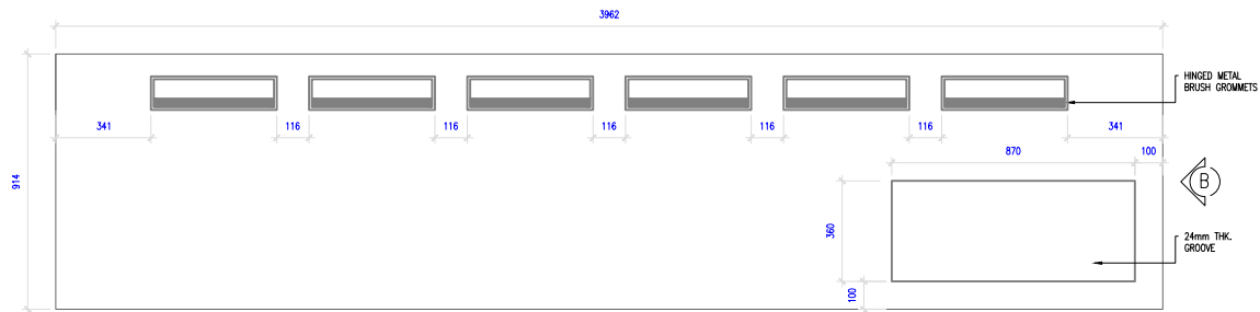
WORK DESK TOP VIEW SCALE: 1:15
