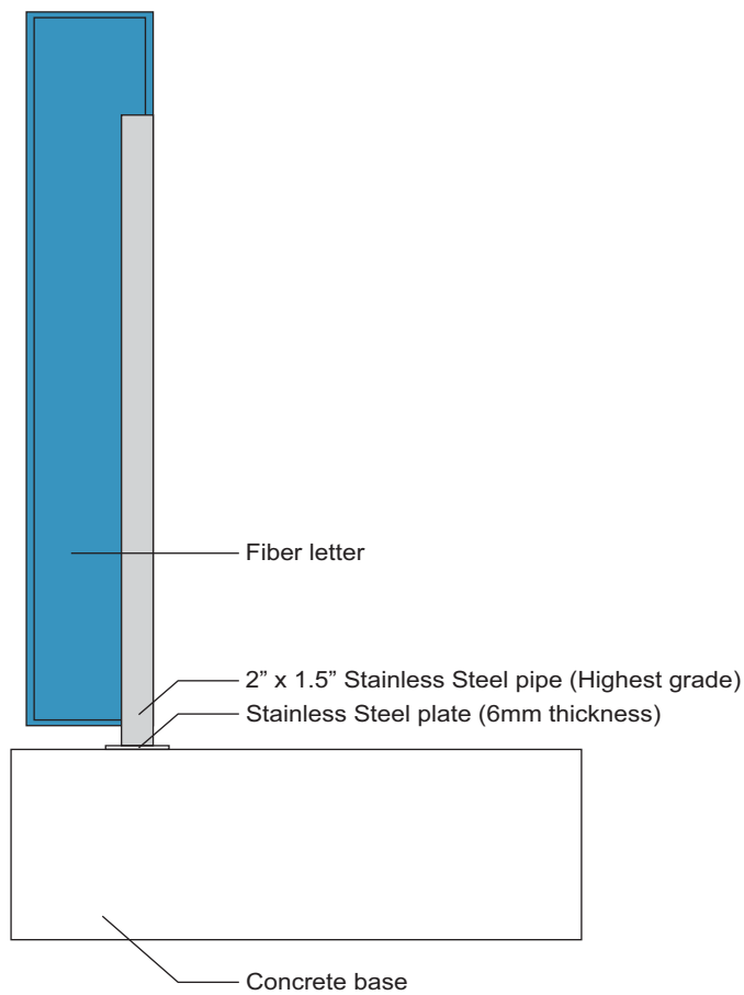
SIDE ELEVATION
