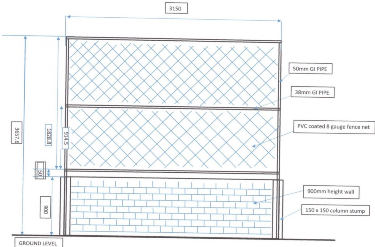
FENCING DETAIL
