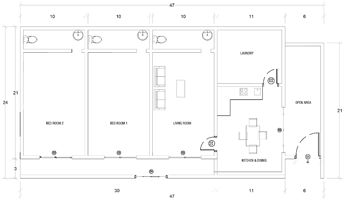
2 ROOM APARTMENT FLOOR PLAN
