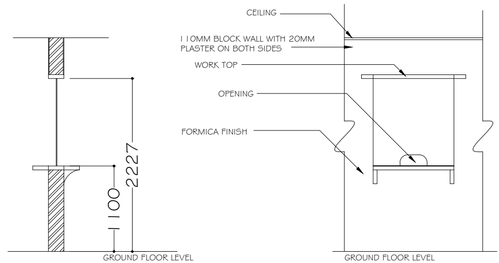
COUNTER DETAIL 1:50
