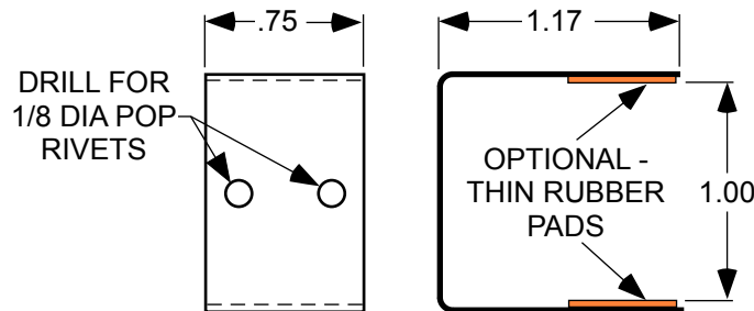
LATERAL BATT RETAINER
