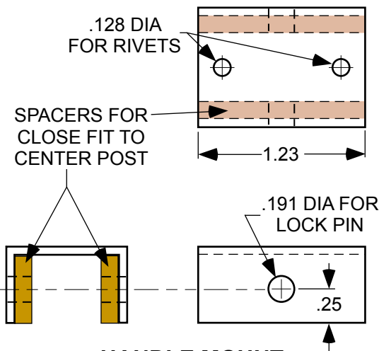
HANDLE MOUNT
