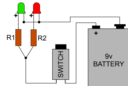
ELECTRONIC CIRCUIT LAYOUT
