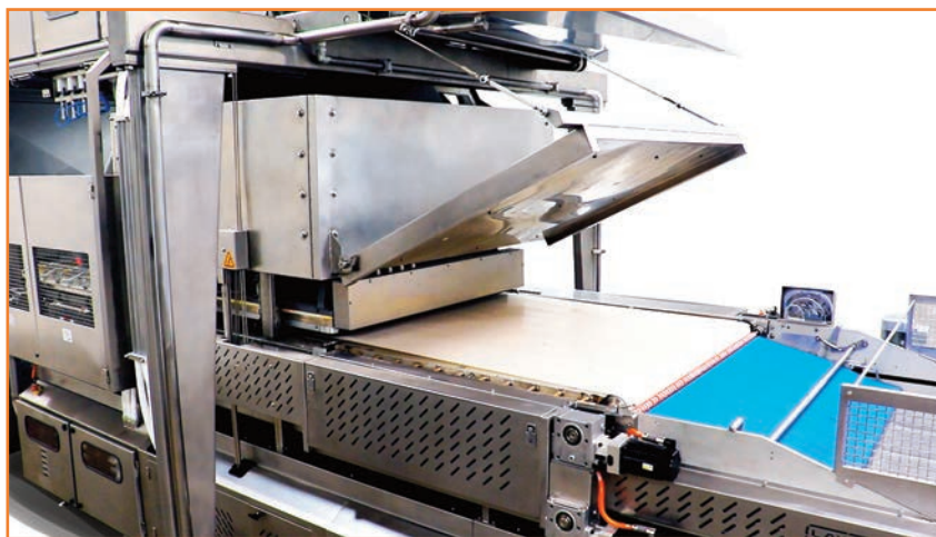
Complete press head insulated enclosure with electric lift system
