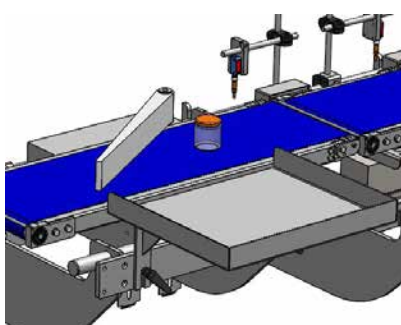
Diverting arm
