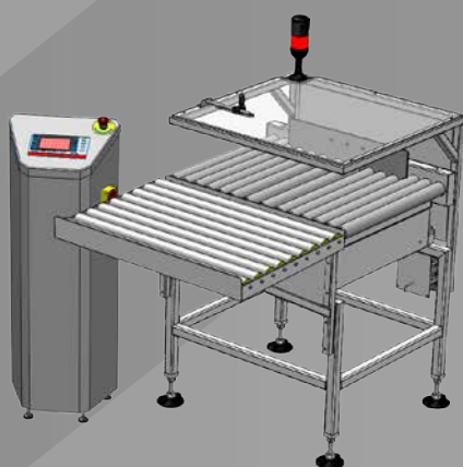
Rejection on the weighing belt
