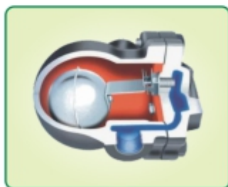
AIR / GAS ELIMINATOR
