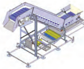
Z CONVEYORS
