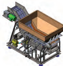
HOPPERS
