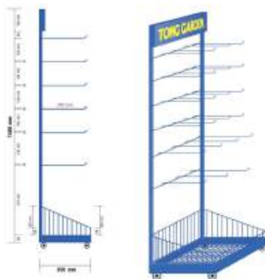
▲ Rack Display
