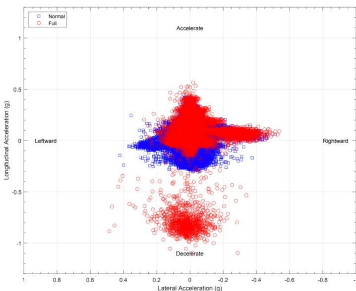
Normal versus aggressive driving accelerometer data.
