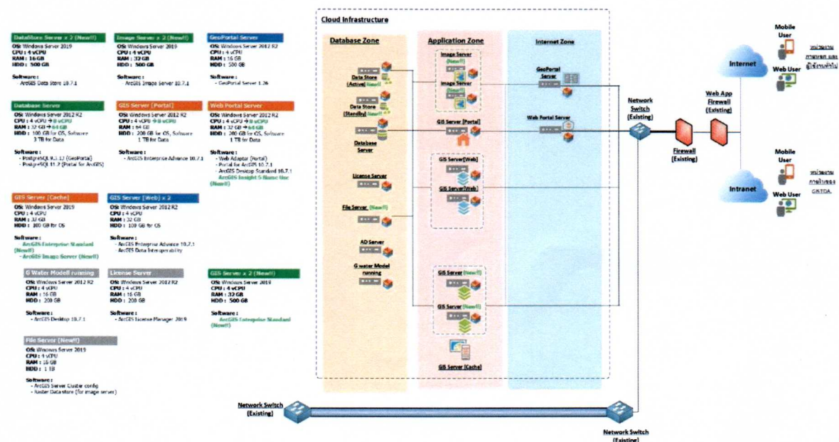
GISTDA GI Portal : System Diagram
