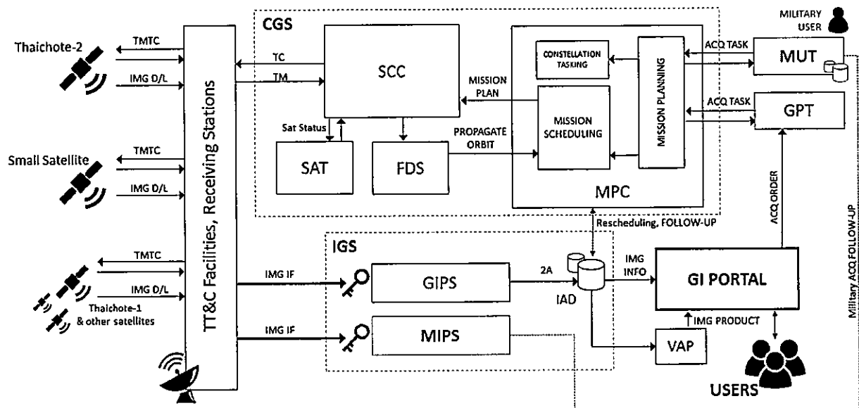
Fig. 13 THEOS-2 satellites operation ground segment
