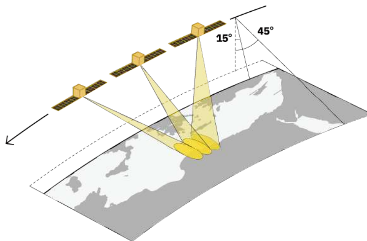
Figure 2.2 Sliding Spotlight mode
