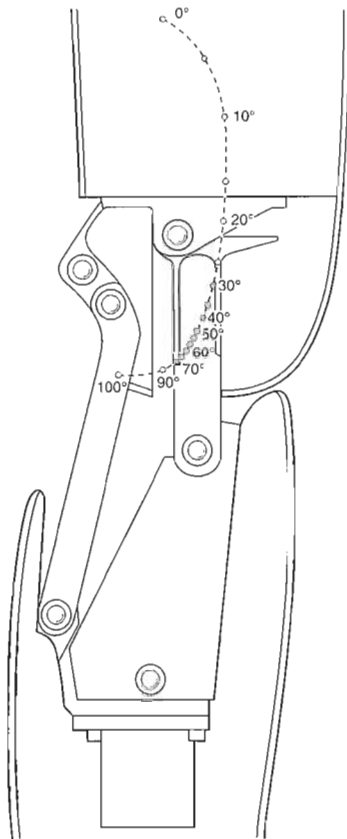
FIGURE 30-26. Four-bar-linkage is an internal polycentric knee that provides many advantages to the patient, e.g., increased stability and better ground clearance during swing phase. As indicated in this illustration, the point of rotation varies with the degree of flexion. With the knee flexed, the leg folds under the thigh segment, and thus is very useful for longer residual limbs. There is also a hydraulic version of the four-bar linkage for children.
