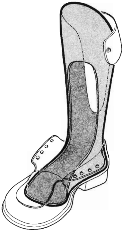
FIGURE 16-20. An ankle-foot orthosis made of a polypropylene shell with a Plastizote lining. The orthosis is closed anteriorly over the tibial tubercle so that the floor reaction force can be transmitted directly to the area of intact sensation. (From ref. 117, with permission.)
