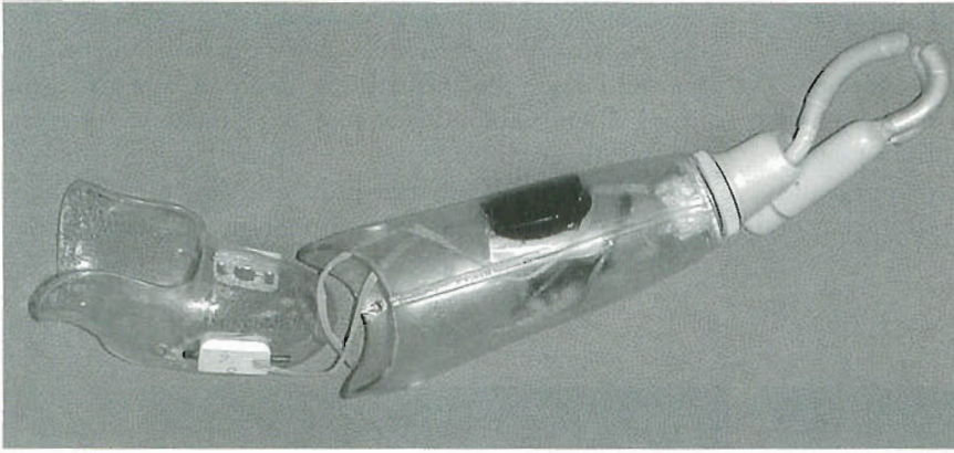
FIGURE 30-19. This example of the myoelectric prosthesis was made with a clear socket for teaching purposes. The proximal portion of the socket, which fits on the residual limb, contains the electrodes that pick up the signals from the muscles. This fits into the prosthesis, which contains the electrical and mechanical working parts of the Otto Bock Electrohand.
