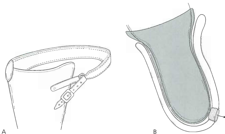
FIGURE 30-22. Methods of suspension for transfemoral prostheses. A: The Silesian belt is almost universally used in the young pediatric patient, to suspend a transfemoral prosthesis, and occasionally a knee disarticulation or transtibial prosthesis (see also Fig. 30-15B). B: The suction socket is a tight-fitting socket design with a one-way valve that allows air to be expelled with weight bearing to maintain a suction fit on the residual limb. It is best suited for the older child or adolescent, who has a mature limb that is not changing in size.
