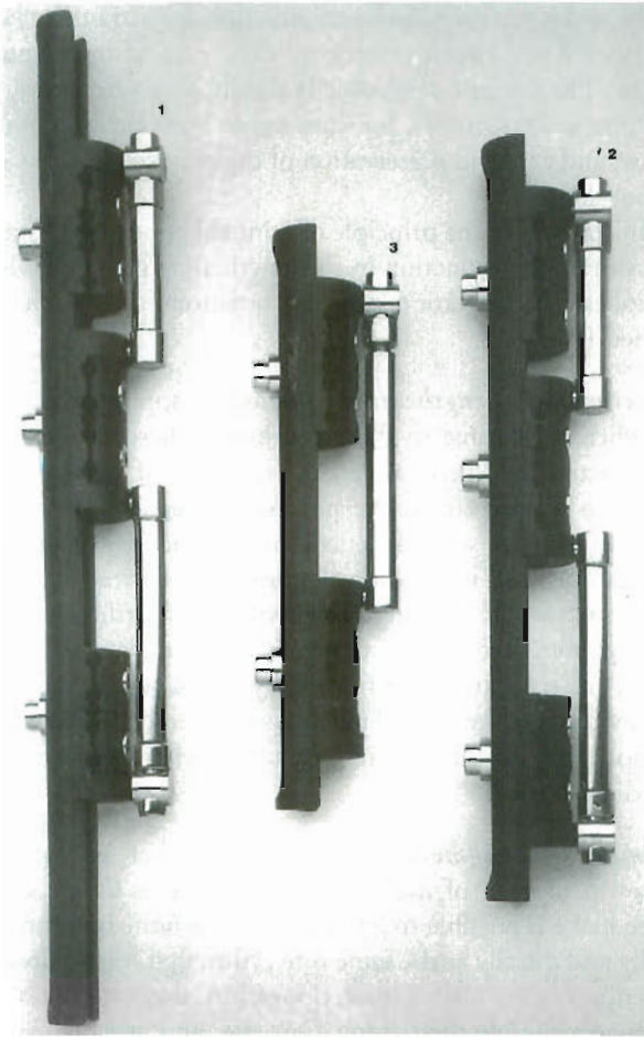
FIGURE 28-32. The Orthofix track lengthening device places the lengthening mechanism beside the pins instead of between them, thereby increasing the excursion and obviating device exchange during lengthening. Like the standard device, it is not adjustable once the pins are in place.
