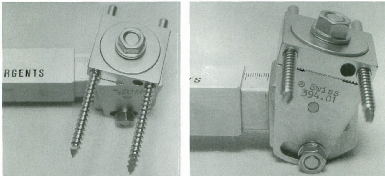
FIGURE 28-31. The Wagner device can be adjusted in two planes, but not in rotation. It allows correction of angulation that develops during lengthening, but does not allow simultaneous lengthening and gradual correction of angular deformity.
