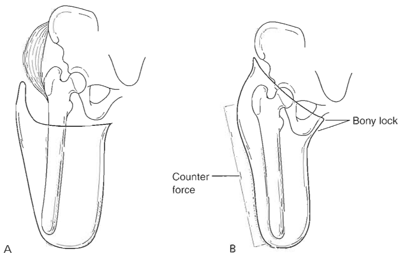
FIGURE 30-21. A: The quadrilateral socket is useful for the young child, especially if end-bearing is possible. However, it fails to stabilize the femoral segment in a transfemoral amputation. B: This has led to the popularity of the narrow medial lateral socket design, e.g., the ischial containment socket shown here. This design can prove impossible in small infants, because of the fatty thigh and buttocks as well as diapers.
