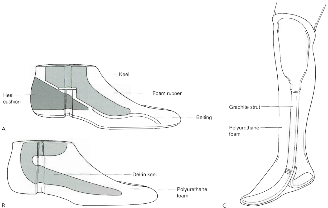
FIGURE 30-27. A: The solid ankle cushion heel (SACH) foot. The length of the keel controls the toe lever arm, and thus the hyperextension moment at the knee, while the compression of the material at the heel absorbs the forces at heel strike. B: The Seattle foot is one of the many varieties of energy-storing feet. It incorporates a flexible keel in the foam foot. This is one of the most common feet used in the pediatric amputee. C: The Flex-foot is another energy-storing foot, but with much different performance characteristics than the Seattle foot. It is used for the older, stronger, and physically active child who has the physical ability to use such a foot.
