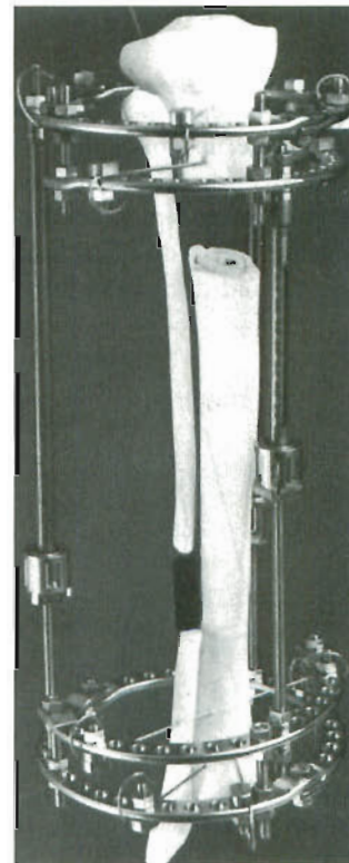
FIGURE 28-33. Ilizarov lengthening device. External fixation is accomplished by tensioned wires fixed to circumferential rings. (From ref. 208, with permission.)
