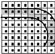
Scan converter decides which pixels to turn on
