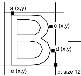
Scaled outline with pixel coordinates
