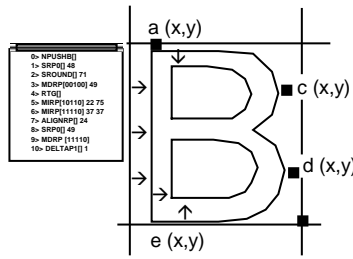
Interpreter executes instructions associated with glyph "B" and gridfits
