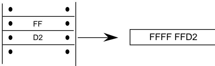
Figure 3–3 A word sign extended to a 32 bit long word (ULONG)
