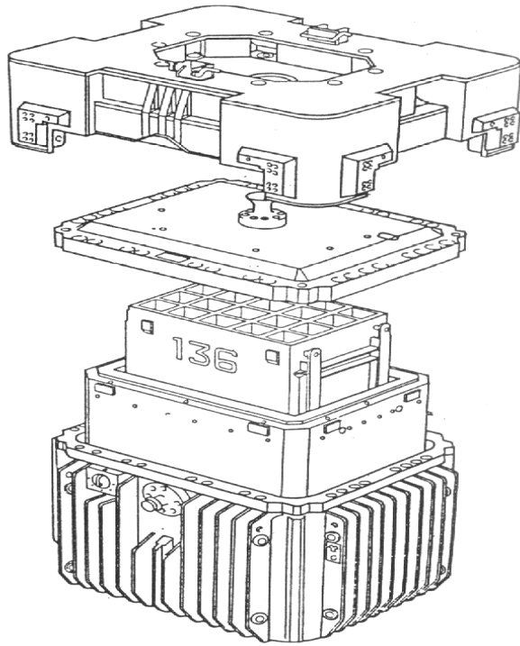
AGR Flask with skip to hold assemblies upright
