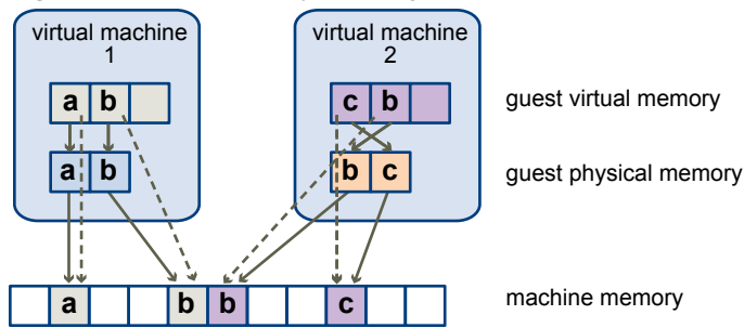
Figure 5-1. ESXi Memory Mapping
