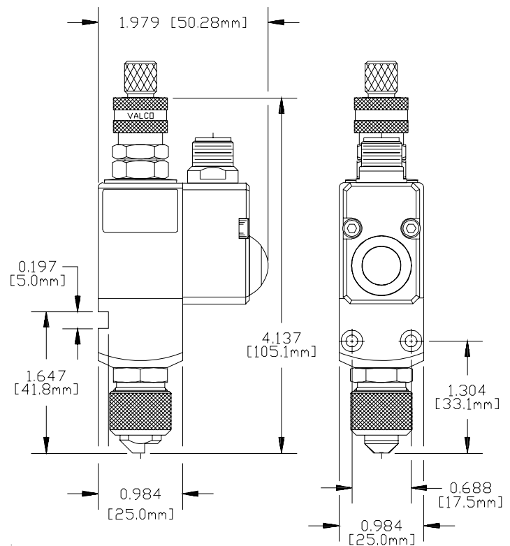
400ECT Valve
