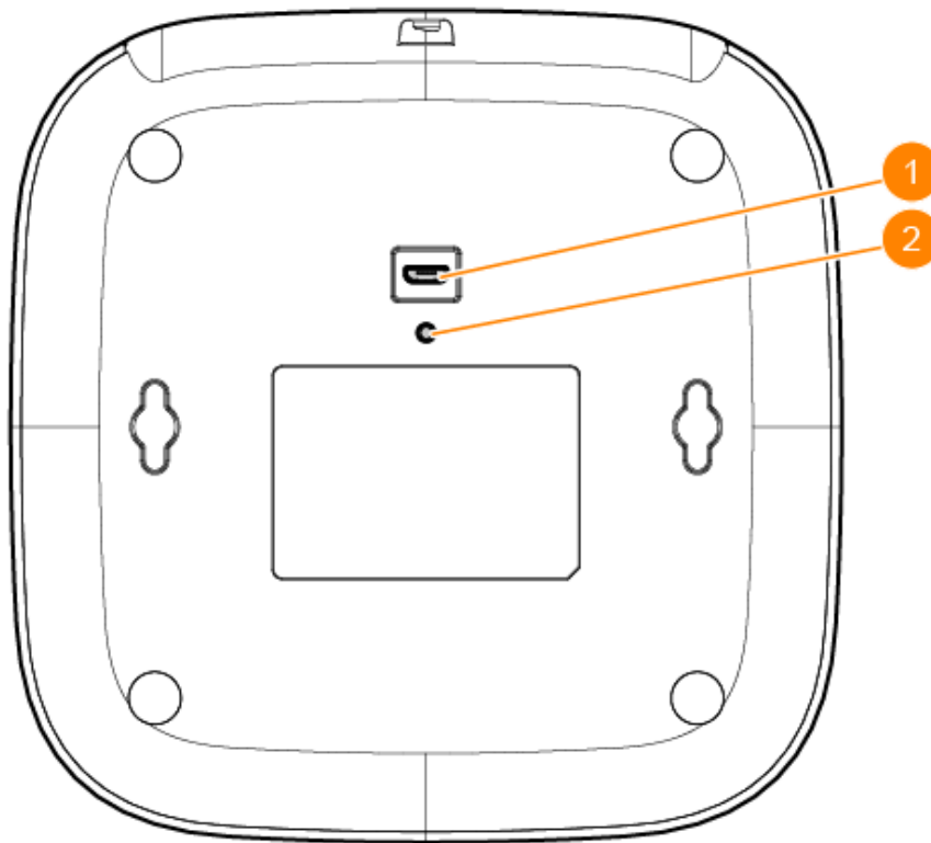
Figure 3 AP-503R Bottom View
