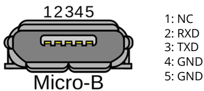
Figure 6 Micro-B Console Port Pin-out
