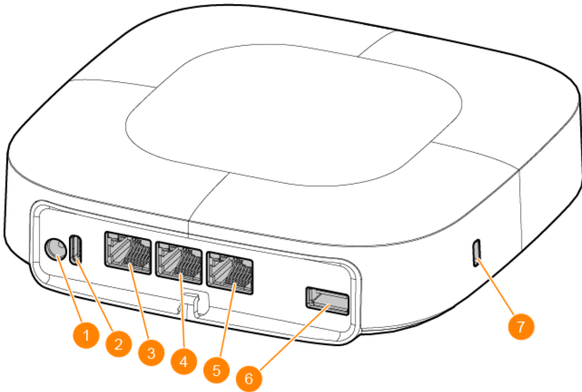
Figure 2 AP-503R Rear and Side View
