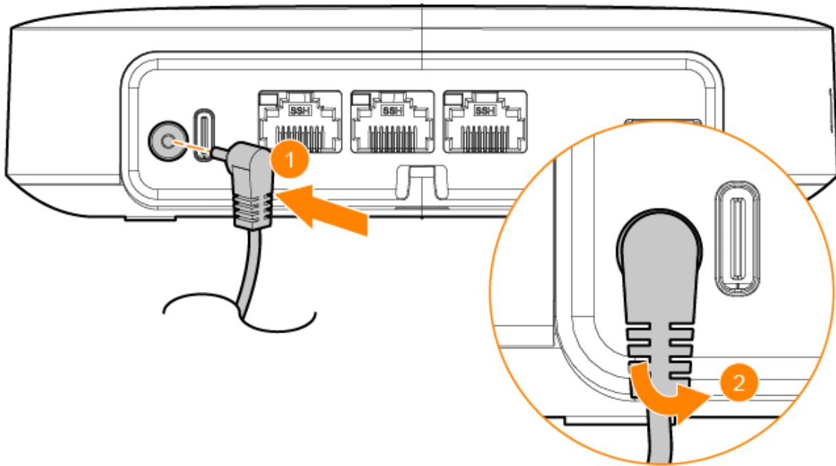
Figure 5 Routing Power Cord through Cable Hook
