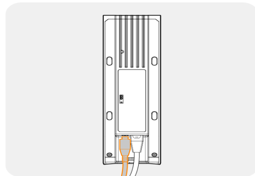
Figure 9 Ethernet + Optional Power Accessory (DC)
