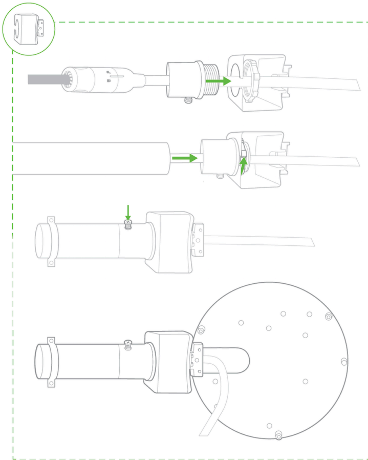
Installing the conduit box to MV93 series: (optional)
