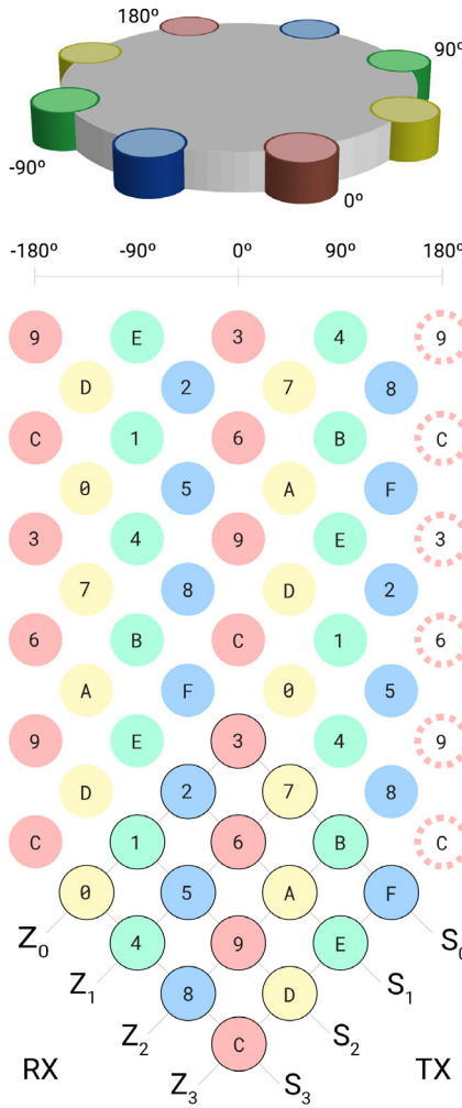
Figure 2. Left) A Helical Sensing Matrix based on a 4x4 braid, which uses 8 conductive threads spiraled around the core. Conductive yarns are shown in color, while support yarns are shown in grey. Z_0 – Z_3 (magenta) are conductive yarns in the Z-direction, which are used as receive lines in the sensing matrix. S_0 – S_3 (cyan) are conductive yarns in the S-direction, which are used as transmit lines in the sensing matrix. Center) Flattened Helical Sensing Matrix, that illustrates the infinite number of 4x4 matrices (colored circles 0-F), which repeat along the length of the cord. Rotation gestures are detected by tracking horizontal finger motion across the columns (red, yellow, green, blue). Right) We can also use fiber optic lines instead of passive yarns, to embed visual feedback in the same topology. Here, four passive yarns have been replaced by fiber optic lines F_0 – F_3 (yellow).
