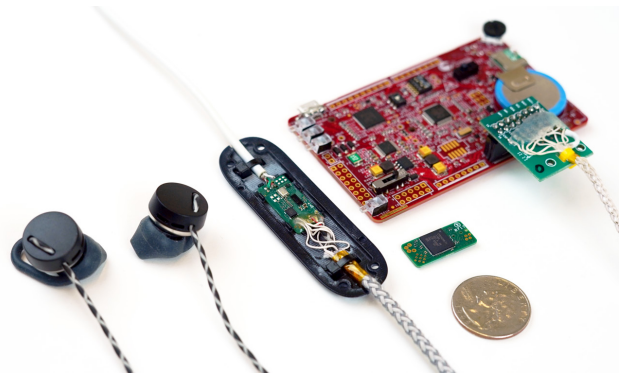
Figure 12. From left to right: (1) I/O Braid USB-C headphones. (2) Nanoboard, custom PCB for 3×3 I/O Braids with onboard tap/gesture sensing and sound tone generation. Configurable as a USB audio interface and as a USB Human Interface Device (e.g., keyboard). (3) 4×4 I/O Braid connected to a PSoC S-Series Pioneer Kit through a custom breakout board.
