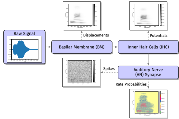
Figure 1: Schematic depiction of an auditory pipeline.
