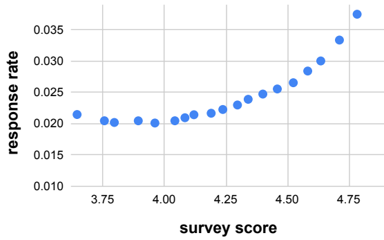
Figure 1: Average response rate (y-axis) vs. satisfaction level quantiles (x-axis).
