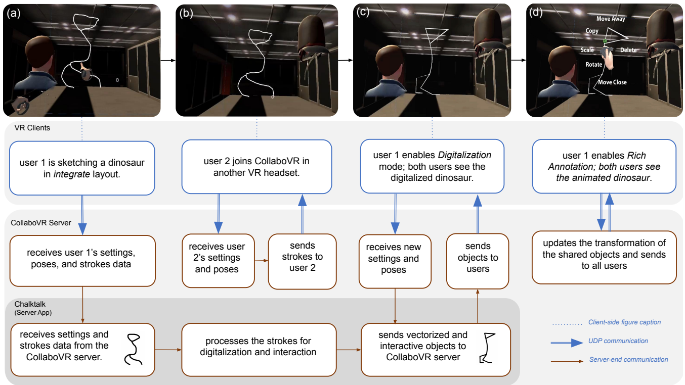
Figure 2: The workflow of CollaboVR: (a) As user 1 sketches in CollaboVR, the server receives the aggregated data of settings, poses and strokes and sends the strokes data to Chalktalk for further processing; (b) When user 2 joins CollaboVR, the server broadcasts the poses from user 1 as well as the latest stroke data so that both users see the sketches and each other; (c) After user 1 triggers the Digitalization mode and notifies the CollaboVR server, the server queries Chalktalk. In less than 16 milliseconds, Chalktalk converts the strokes into interactive objects. Then both users see digital objects (in this case, a triangle and several spline curves) from the CollaboVR server; (d) When user 1 performs Rich Annotation on the sketch, the CollaboVR server alone handles commands for scene editing tasks.
