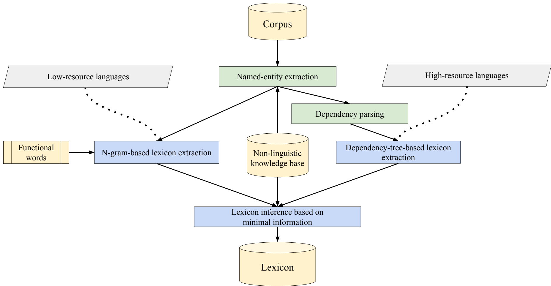
Figure 3: Flow diagram of the proposed architecture for crafting a linguistically annotated lexicon. Note that the lexicon inference based on minimal information is optional.
