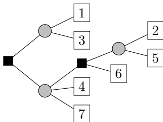
Figure 4: The decomposition tree for a series-parallel circuit.
