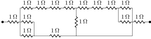
Figure 9: A 15-element approximation of \pi .
