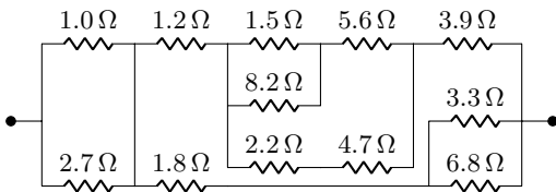
Figure 8: The optimal solution for n = 12 .
