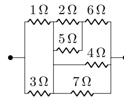
Figure 3: The optimal solution for f_T = \sqrt{7} .
