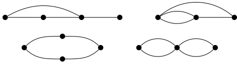
Figure 1: Some series-parallel graphs containing four edges.
