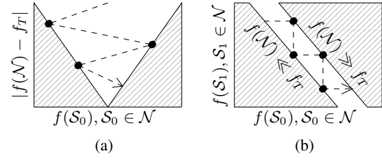
Figure 7: Exploiting convexity via binary search for singleton expandables, or dual linear sweep for expandable pairs.
