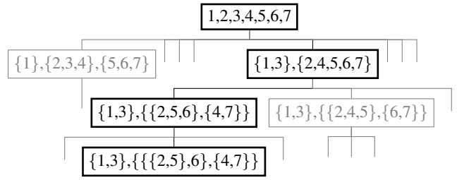
Figure 5: Exploring the space of decomposition trees, with the path to an optimal solution highlighted by nodes in dark.
