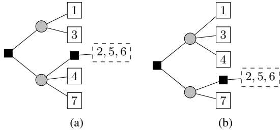
Figure 6: Two distinct decomposition trees that contain the same expandable node.
