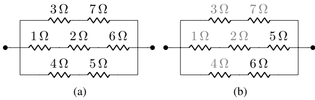
Figure 2: Two circuits composed of the resistors 1 Ω to 7 Ω.
