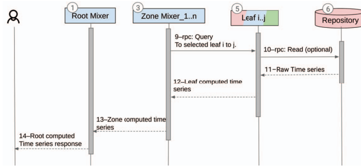
(b) Sequence diagram: the Query pass
