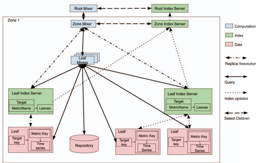
Fig. 2: Box-and-line model of the proposed architecture
