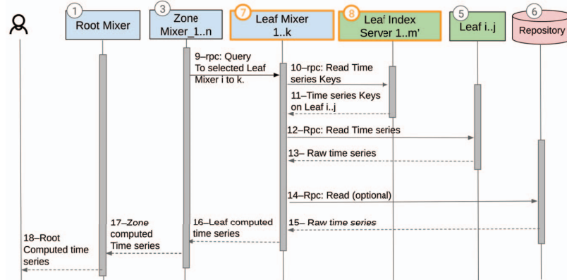
(b) Sequence diagram: the Query pass
