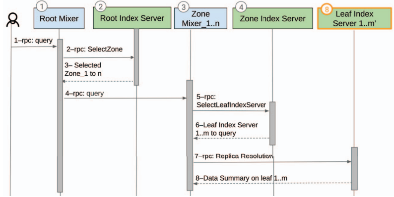
(a) Sequence diagram: the Replica Resolution pass
